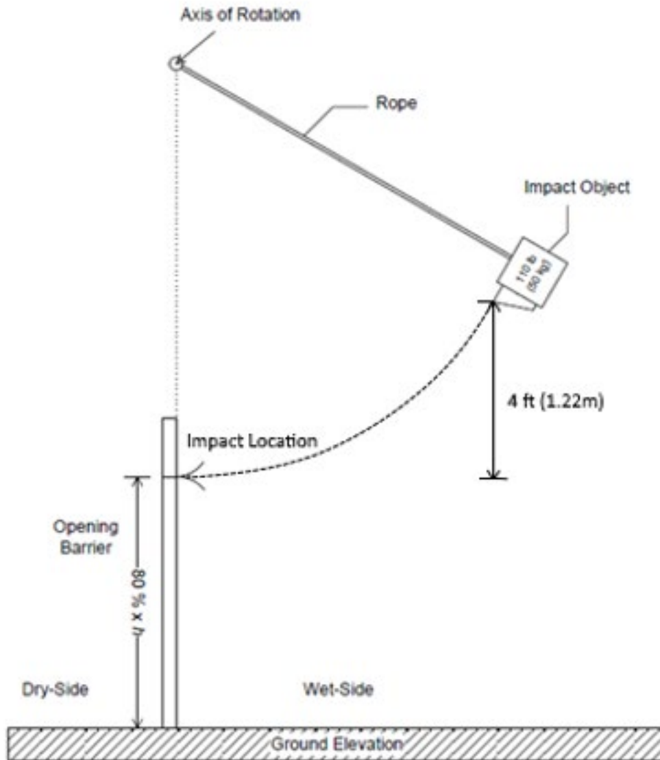
Figure 4.3.4 Impact Test Layout
