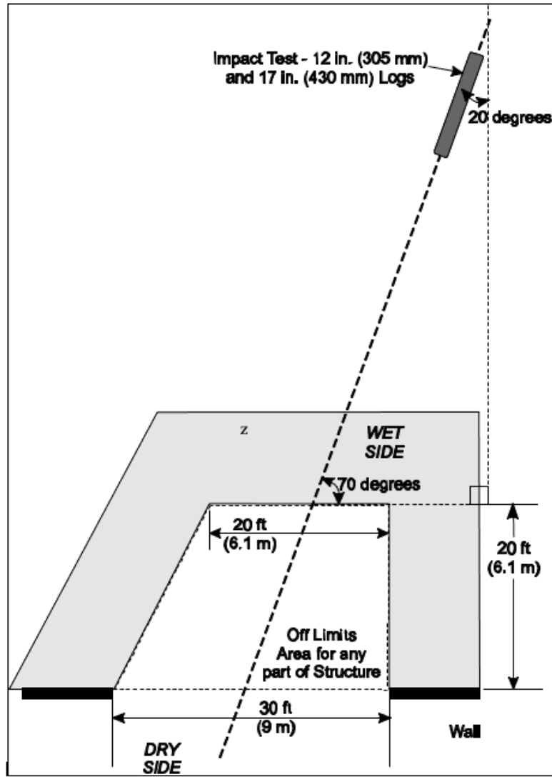
Figure 4.2.5.2 Debris Impact Test Layout
