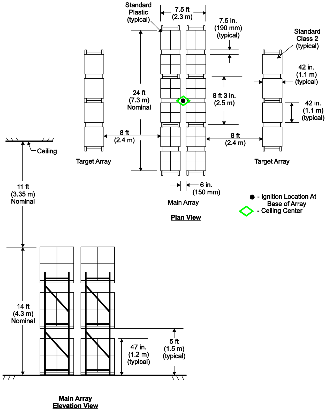
D-34: Full Scale Fire Test Array for K16.8 (K240) Upright Storage Sprinkler, Test B
