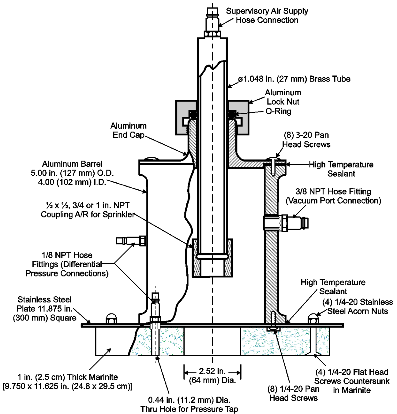
D-10: Modified Plunge Tunnel Test Plate (For Sensitivity Test - Recessed, Flush and Concealed Sprinklers)
