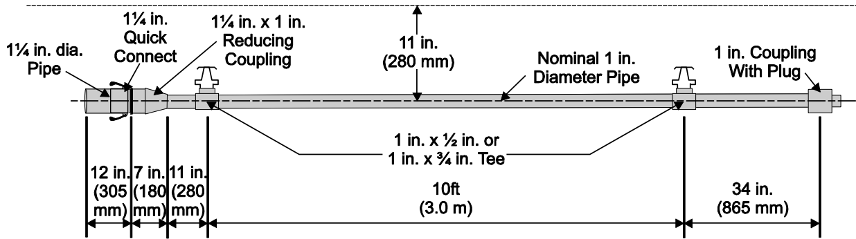
Typical Branch Line
