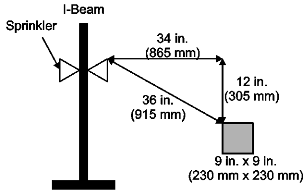
End Elevation View 9 in. (230 mm) Wide Obstruction 36 in. (915 mm) Separation
