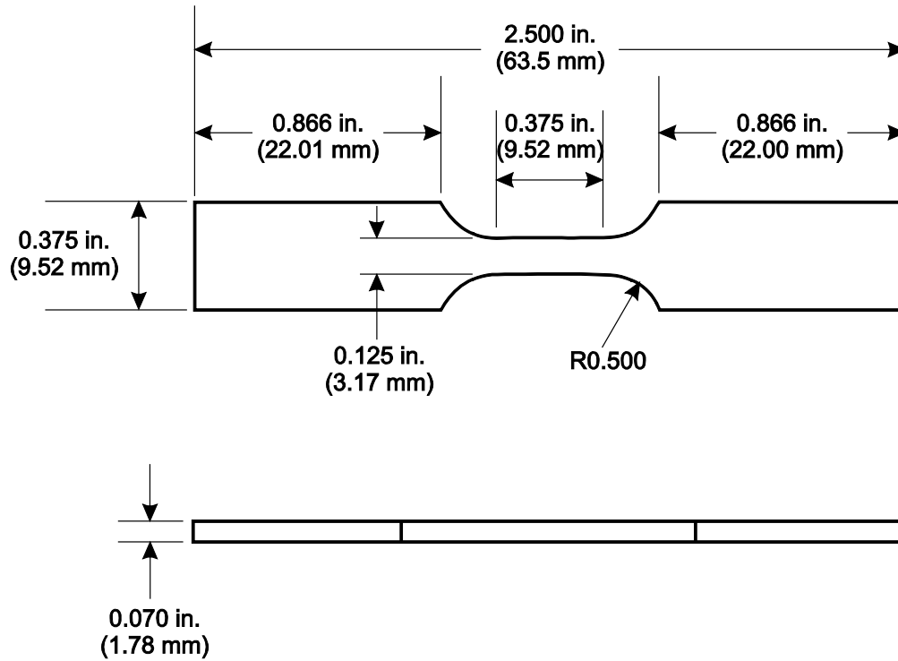
Figure I-2-1 - Schematic drawing for dimensions of Type V tensile specimens in accordance with ASTM D638 of NPS 1 (DN 25) CPVC in accordance with ASTM F442 (units in inches).
