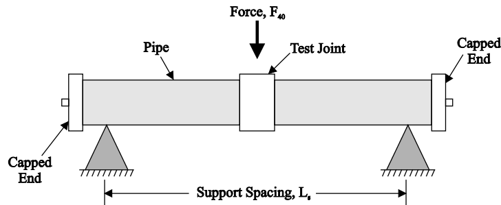
Figure D-2. Bending Moment Resistance Test
