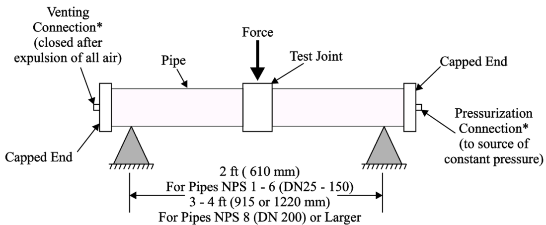
Figure C-2. Bending Moment Test
