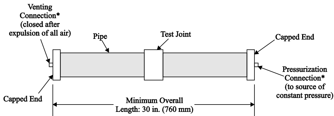
Figure C-1. Hydrostatic Test Sample
