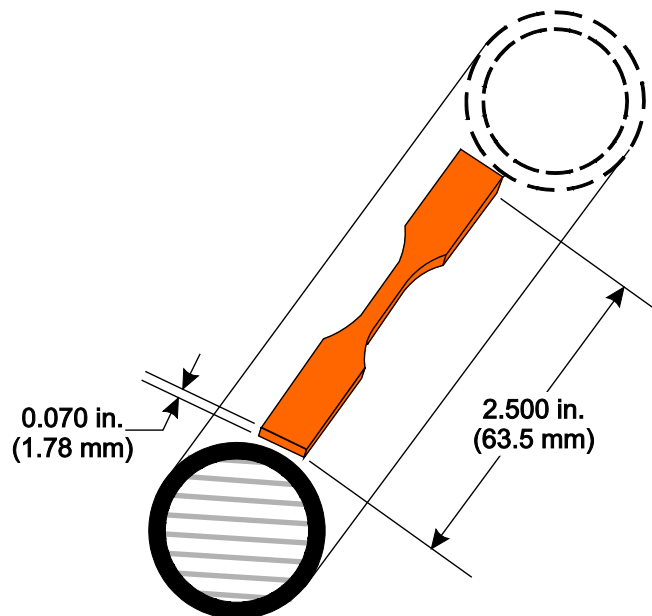
Figure I-2-2 - Schematic drawing for the machining direction of the Type V tensile specimen in accordance with ASTM D638 of NPS 1 (DN 25) CPVC pipe in accordance with ASTM F442 (units in inches).
